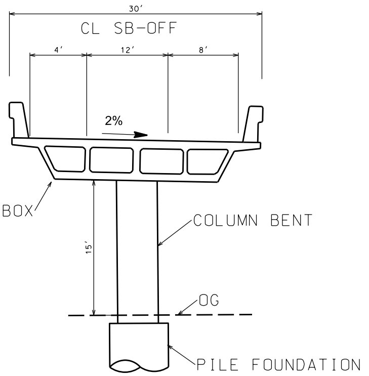
TYPICAL SECTION SB OFF-RAMP PLANNING STUDY
