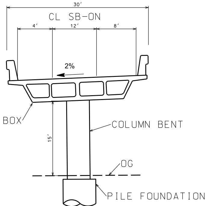
TYPICAL SECTION SB ON-RAMP PLANNING STUDY
